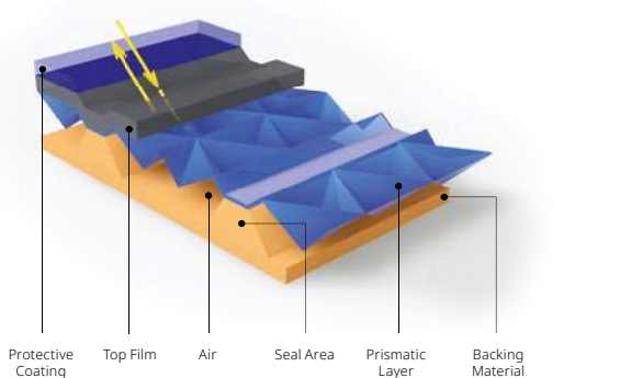
Prismatic Air-backed Construction
